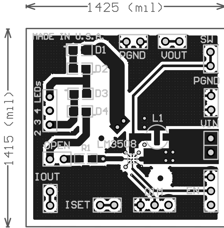
FIGURE 1. LM3508 Evaluation Board Layout Topside
